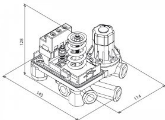
Dimensions PMA/12RP
